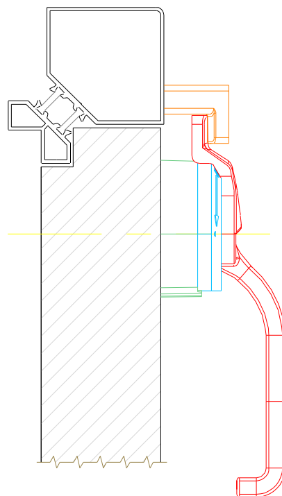
DN ISO - O Double panel, Thermal break profile
